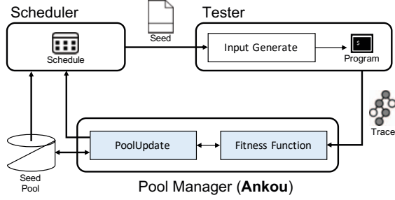
Figure 2: Ankou architecture.
